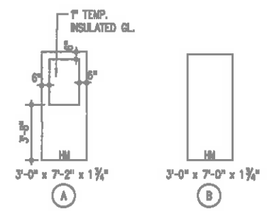
DOOR SCHEDULE \frac{1}{4}'' = 1'-0'' 0 1 2 4 8 12
