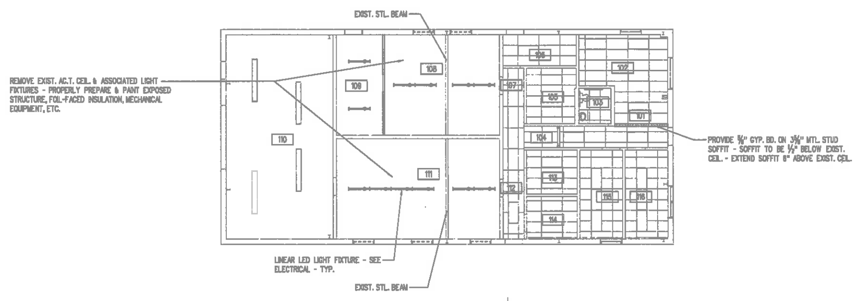
REFLECTED CEILING PLAN \frac{1}{8}'' = 1'-0''
