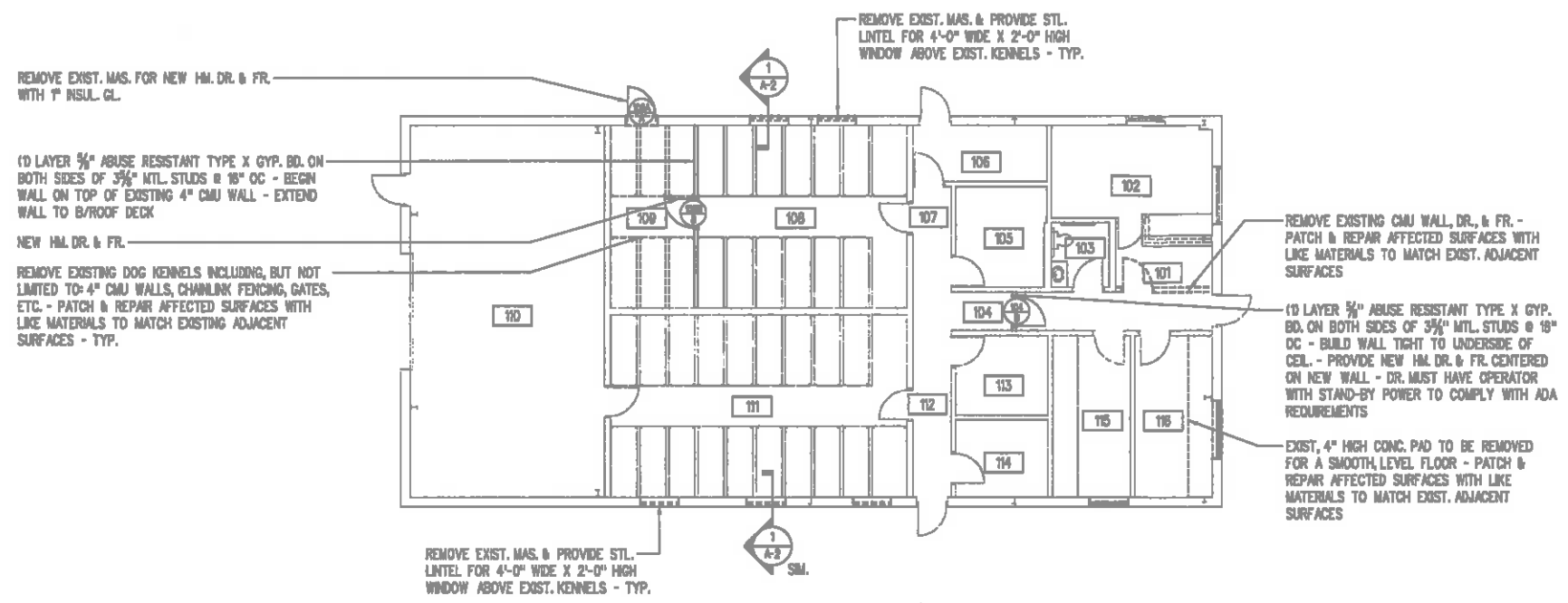
FLOOR PLAN \frac{1}{8}'' = 1'-0'' 0 2 4 8 16 24
