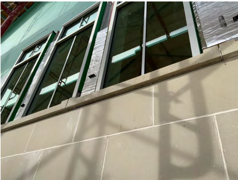
S.S. Flashing and Cast Stone Sill Lugs on South
